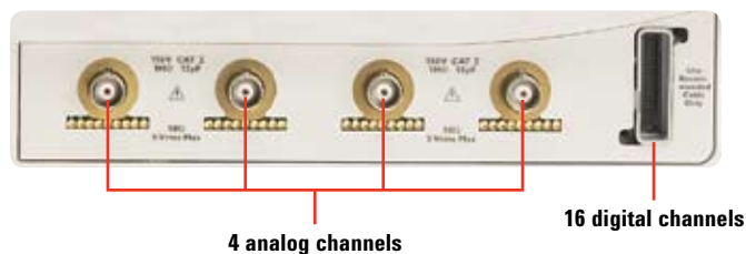
Figure 25. Analog and digital channels on an Agilent MSO 8000 Series oscilloscope
