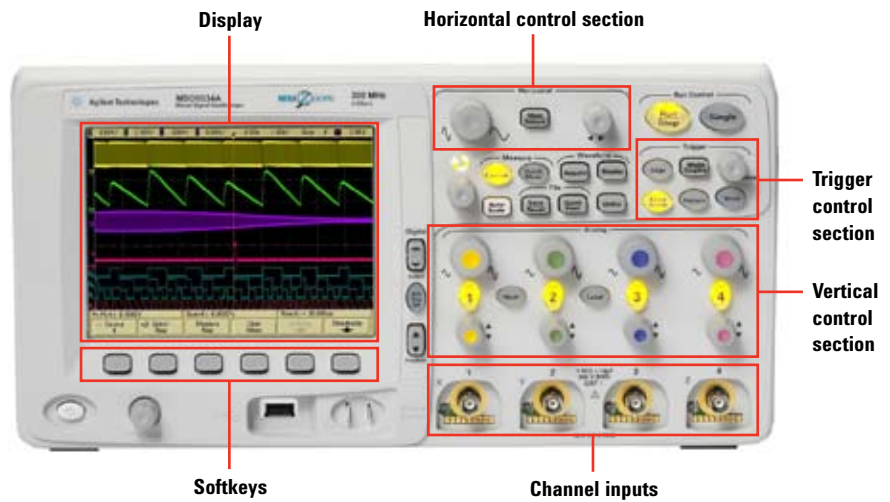
Figure 8. Front panel on the Agilent InfiniVision 5000 Series oscilloscope
